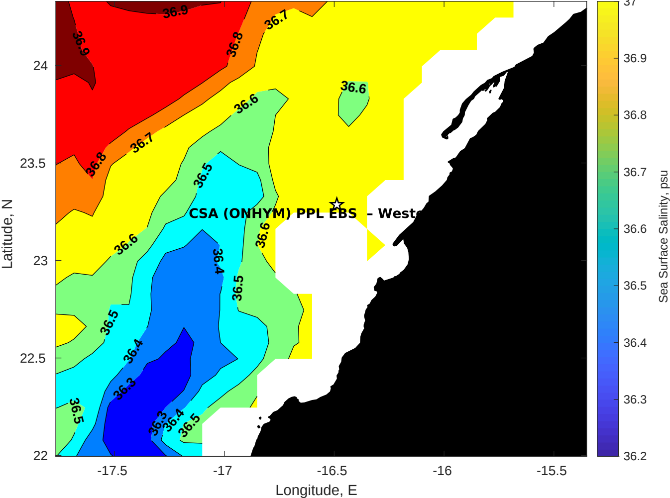
Surface Salinity for CSA (ONHYM) PPL EBS - Western Sahara at 10-Jan-2026 00:00:00
