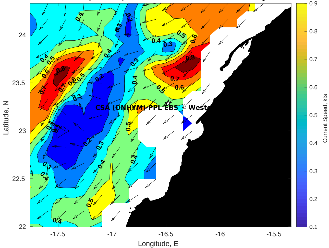
Surface Currents for CSA (ONHYM) PPL EBS - Western Sahara at 10-Jan-2026 00:00:00
