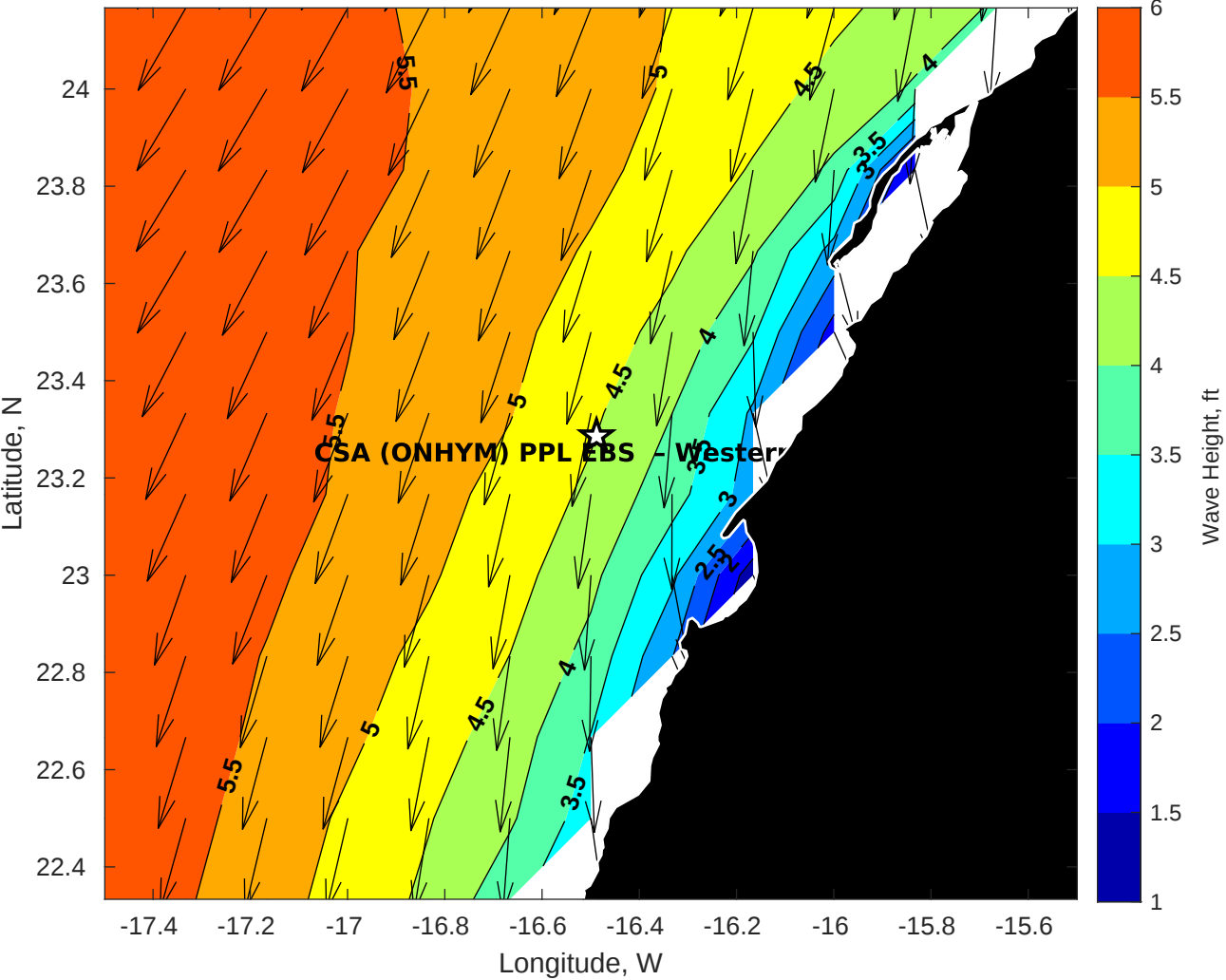
GFS Wave Height (ft) for CSA (ONHYM) PPL EBS - Western Sahara at 11-Jan-2026 09:00:00
