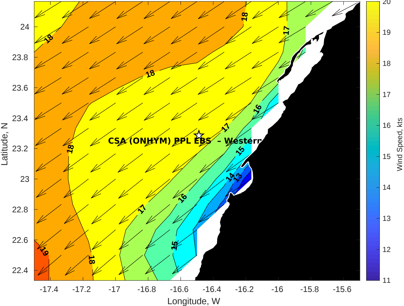
GFS Winds (kts) for CSA (ONHYM) PPL EBS - Western Sahara at 11-Jan-2026 09:00:00
