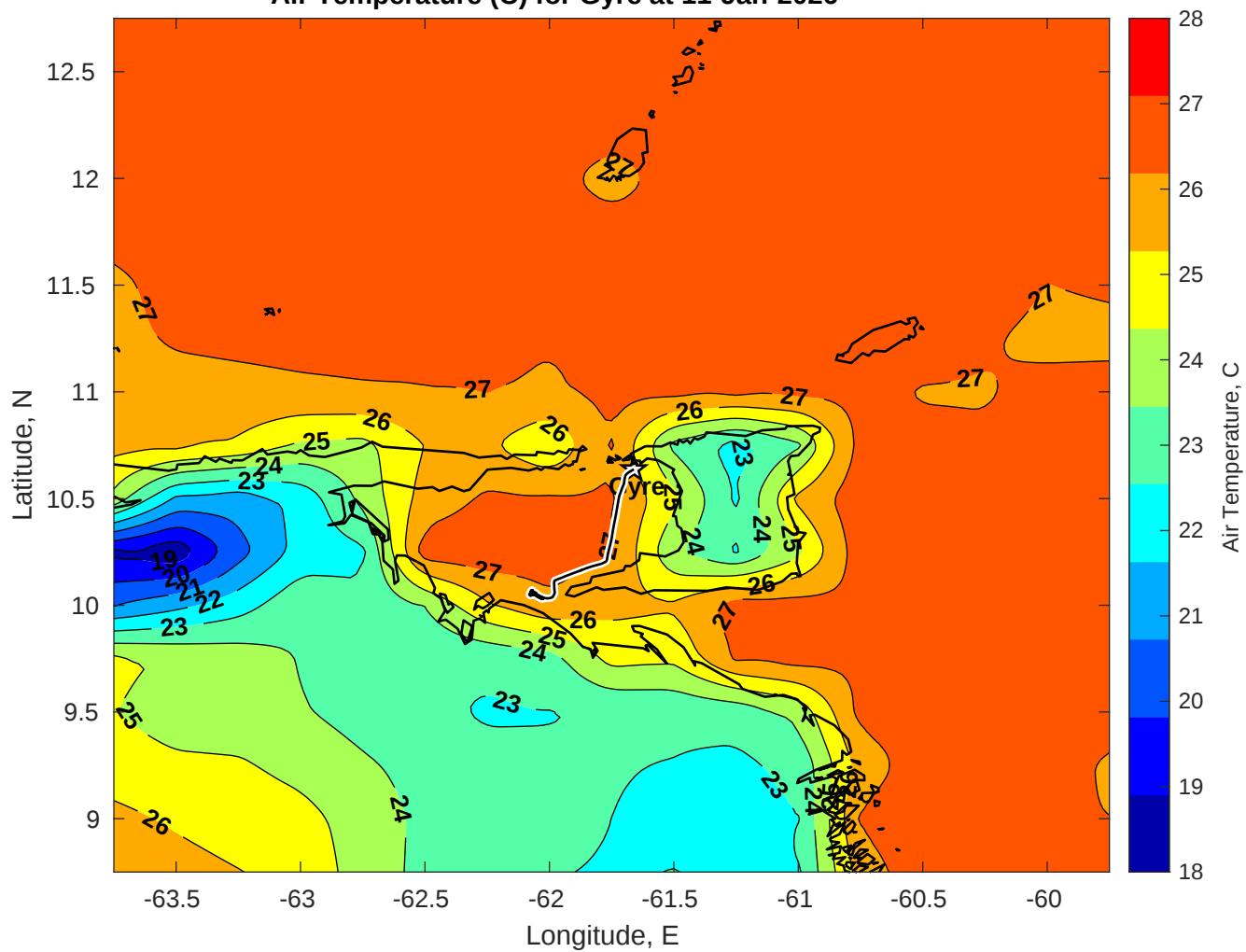
Air Temperature (C) for Gyre at 11-Jan-2026
