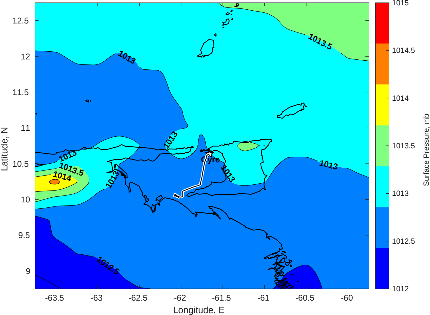
Surface Pressure (mb) for Gyre at 13-Jan-2026 00:00:00
