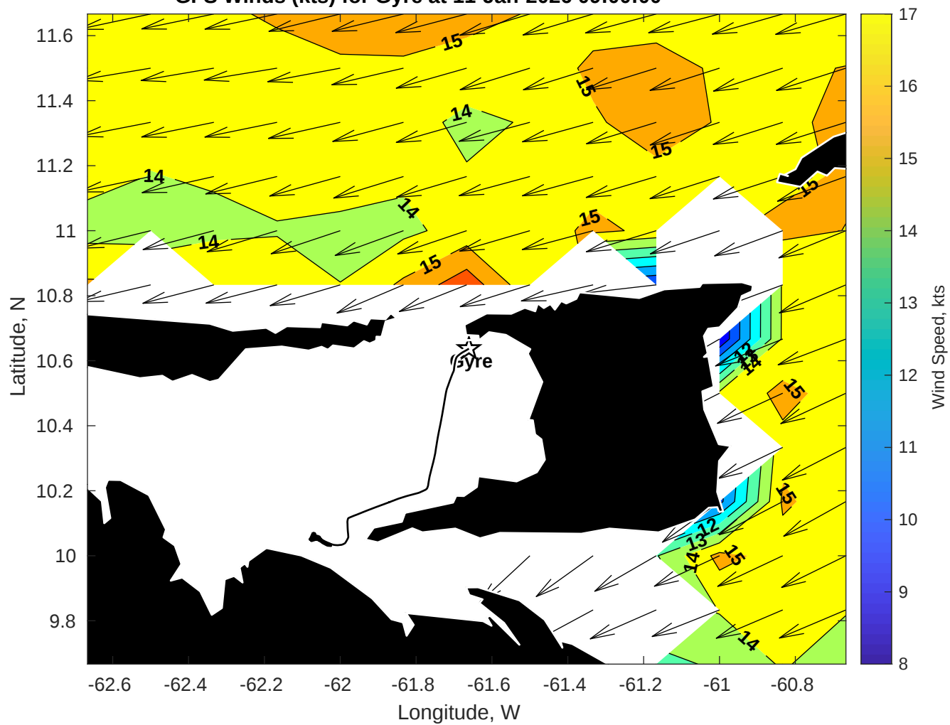
GFS Winds (kts) for Gyre at 11-Jan-2026 09:00:00
