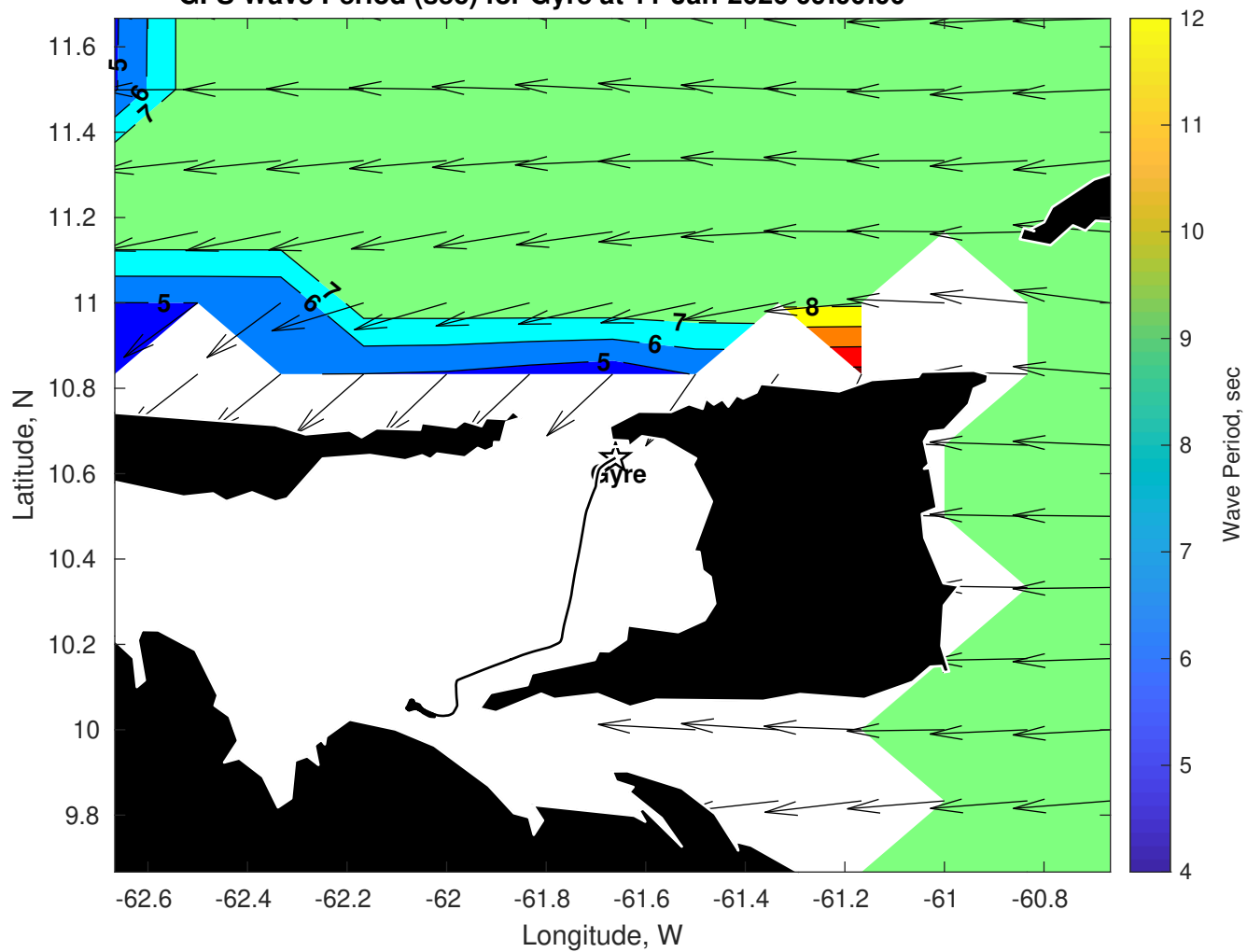
GFS Wave Period (sec) for Gyre at 11-Jan-2026 09:00:00
