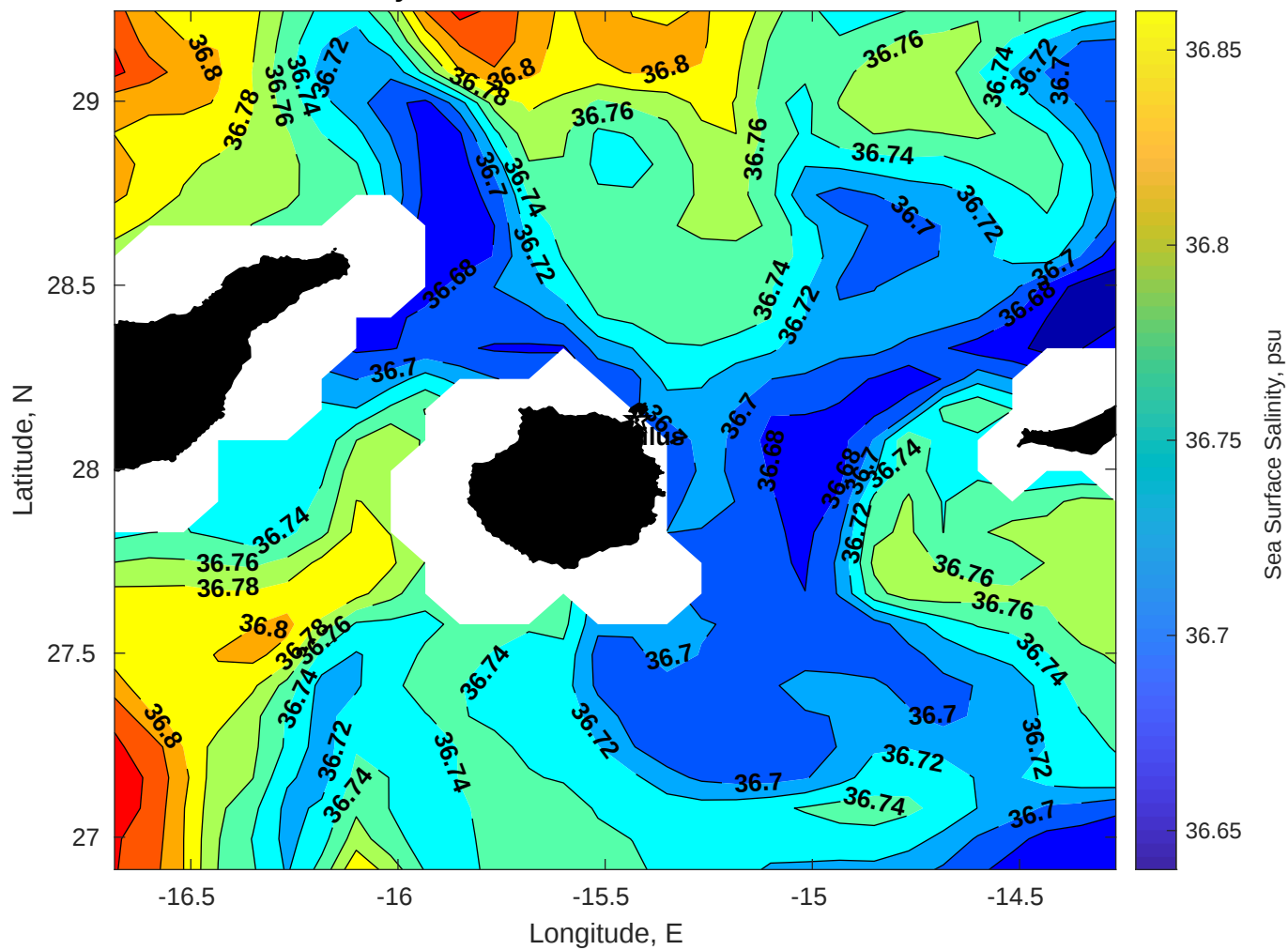
Surface Salinity for Nautilus at 10-Jan-2026 00:00:00
