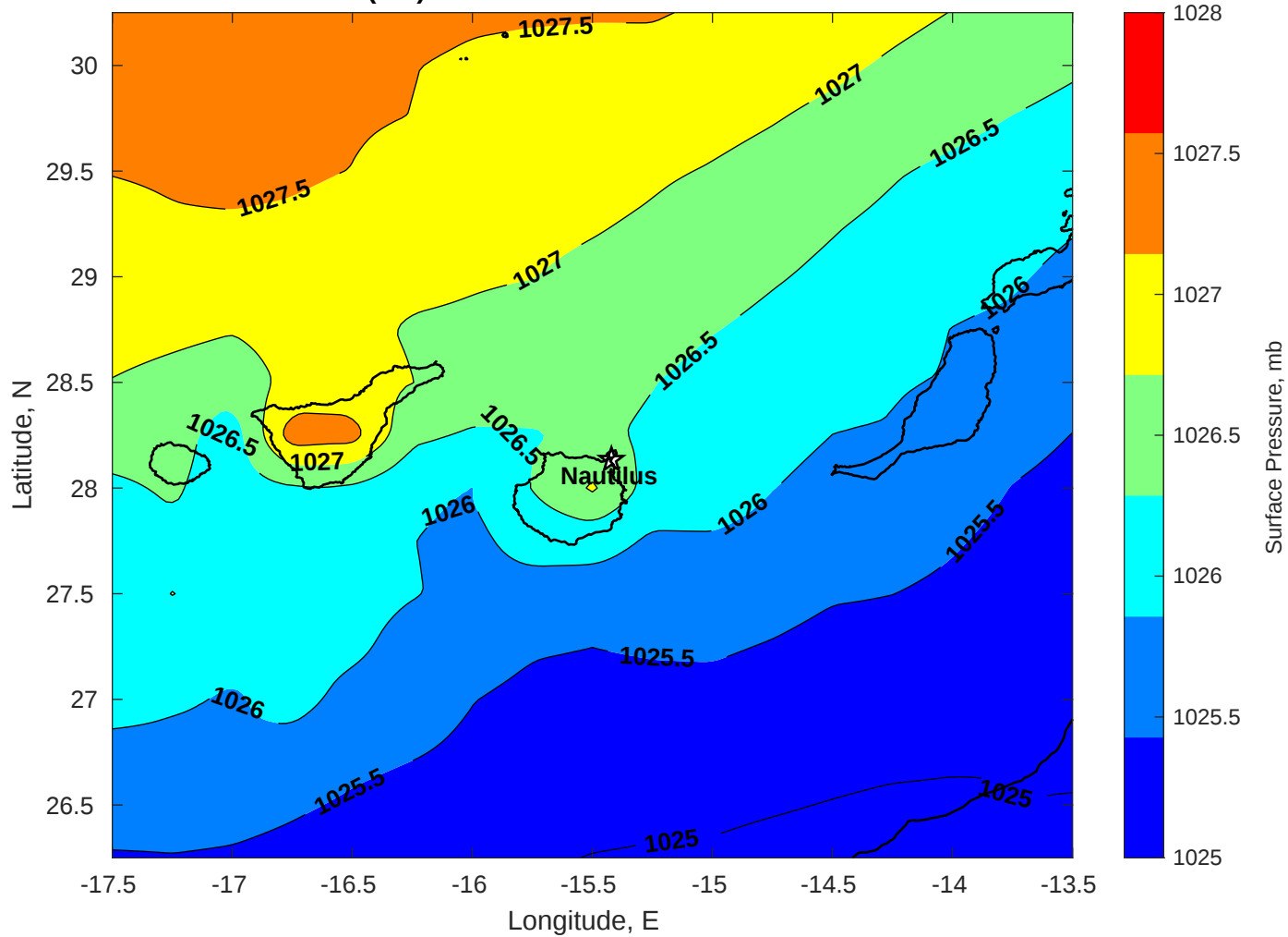
Surface Pressure (mb) for Nautilus at 11-Jan-2026 00:00:00
