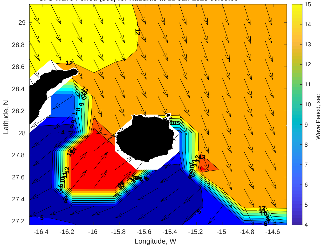
GFS Wave Period (sec) for Nautilus at 11-Jan-2026 09:00:00
