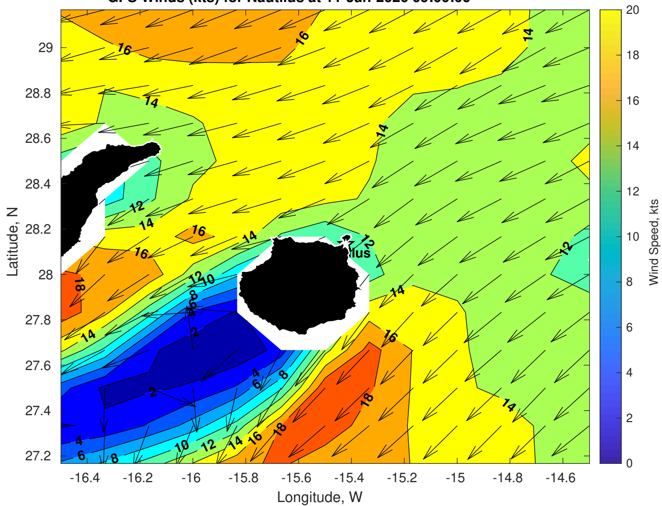
GFS Winds (kts) for Nautilus at 11-Jan-2026 09:00:00
