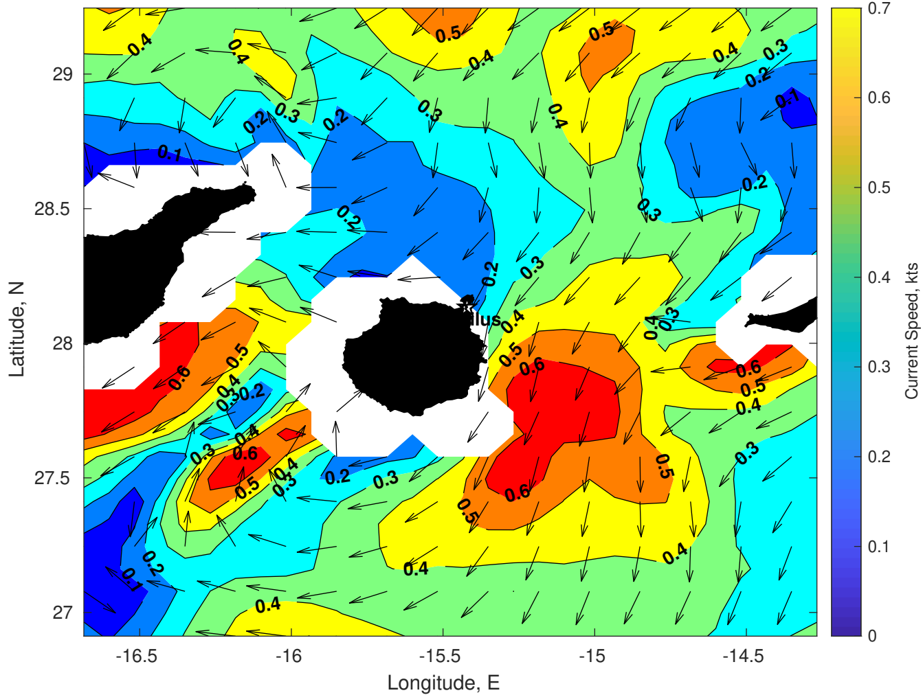
Surface Currents for Nautilus at 10-Jan-2026 00:00:00
