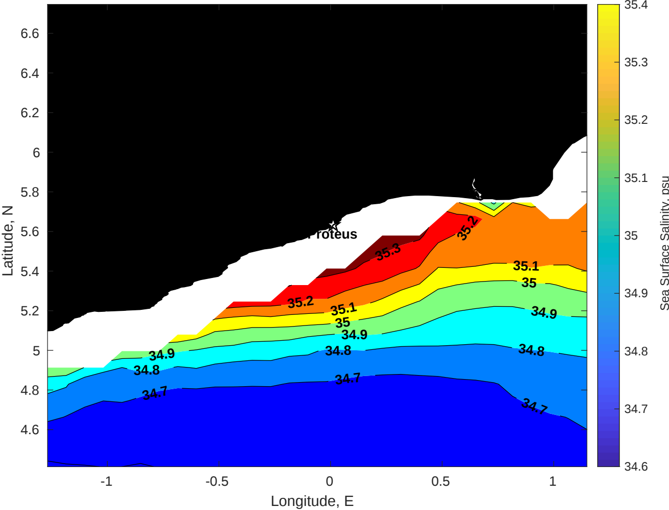
Surface Salinity for Proteus at 10-Jan-2026 00:00:00
