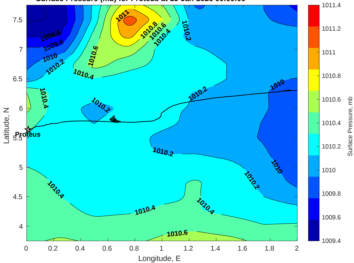
Surface Pressure (mb) for Proteus at 13-Jan-2026 00:00:00
