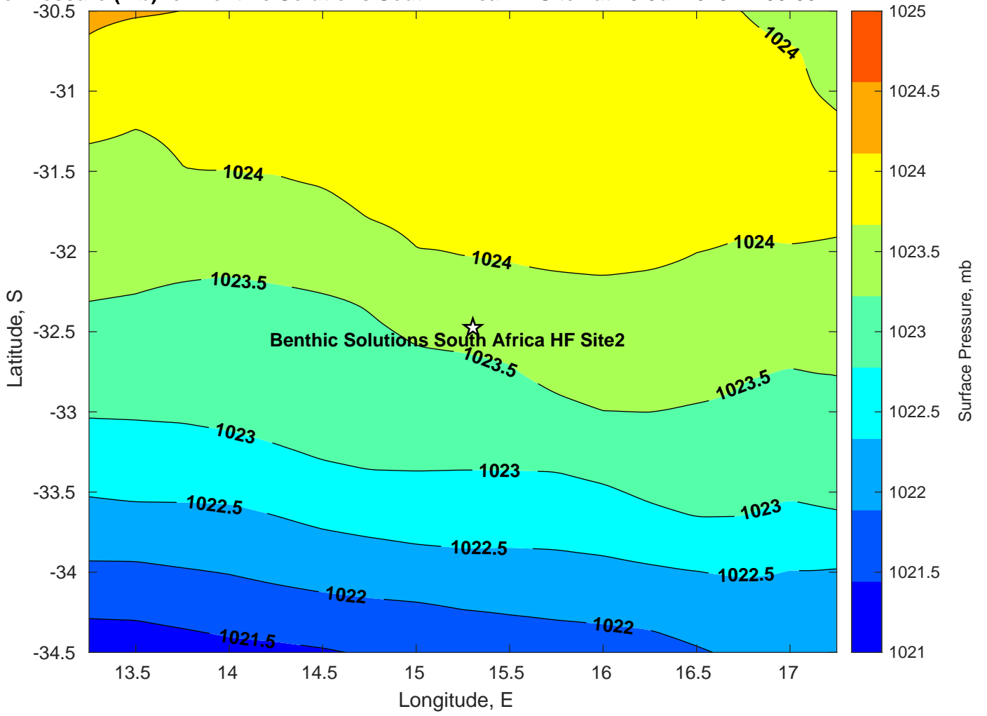
Surface Pressure (mb) for Benthic Solutions South Africa HF Site2 at 13-Jul-2025 12:00:00
