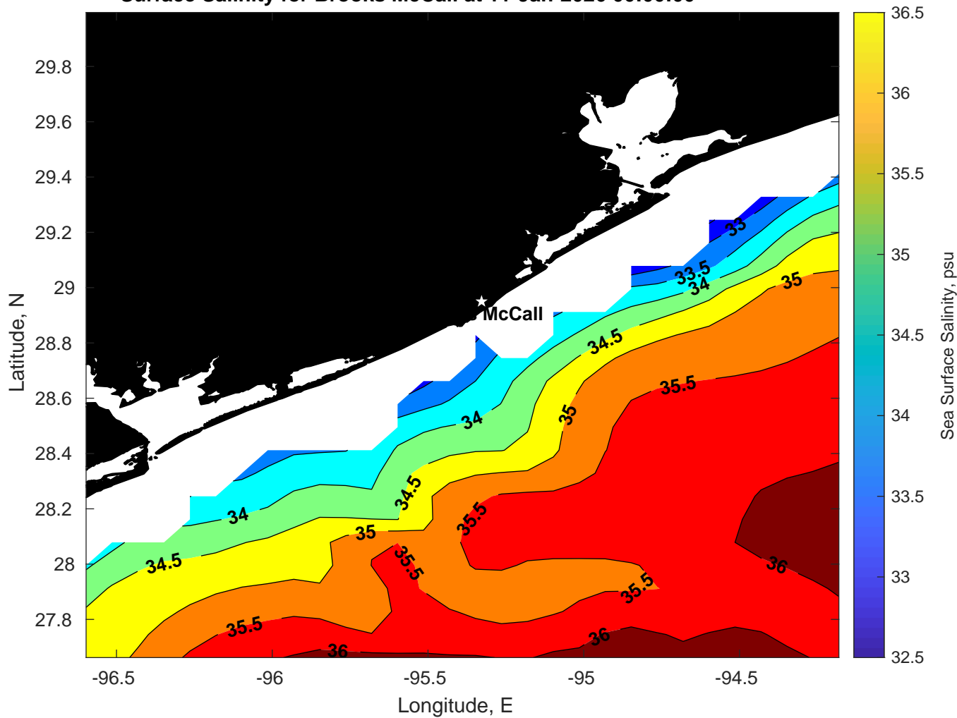
Surface Salinity for Brooks McCall at 11-Jan-2026 00:00:00
