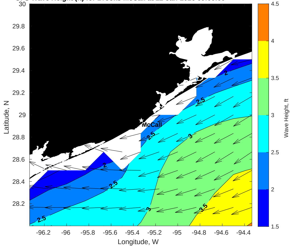
GFS Wave Height (ft) for Brooks McCall at 12-Jan-2026 09:00:00
