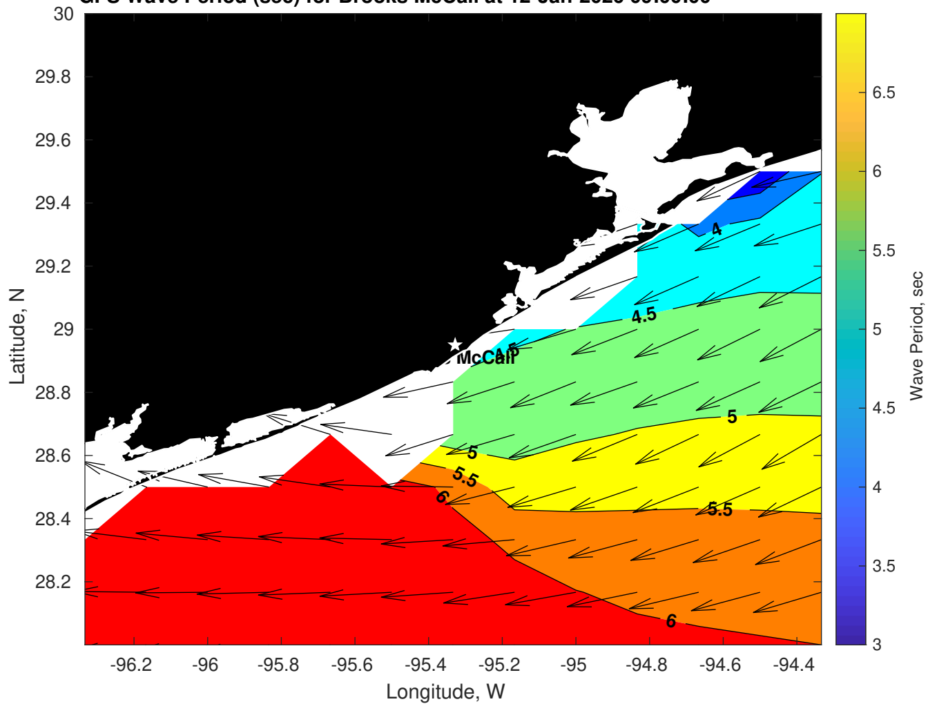
GFS Wave Period (sec) for Brooks McCall at 12-Jan-2026 09:00:00
