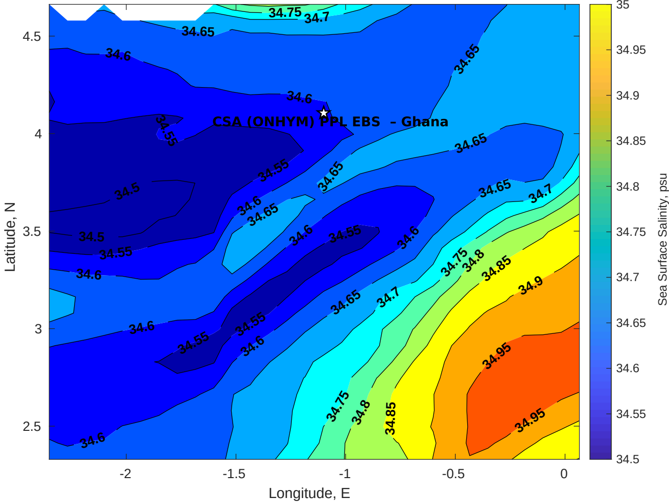
Surface Salinity for CSA (ONHYM) PPL EBS - Ghana at 11-Jan-2026 00:00:00
