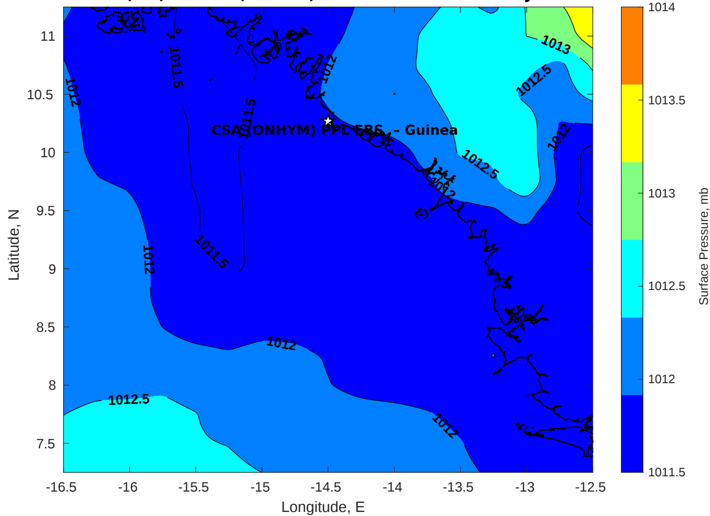
Surface Pressure (mb) for CSA (ONHYM) PPL EBS - Guinea at 14-Jan-2026 00:00:00
