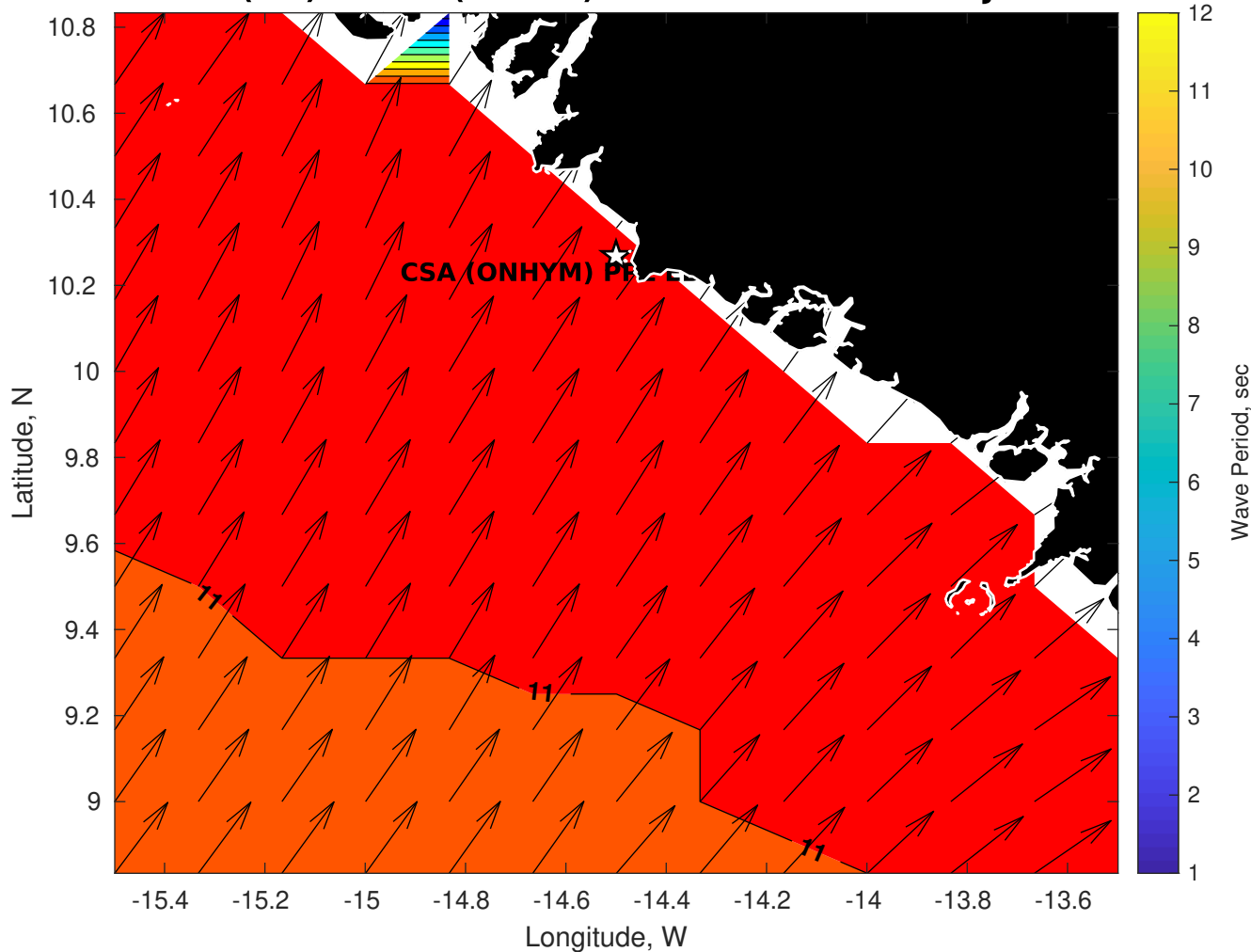
GFS Wave Period (sec) for CSA (ONHYM) PPL EBS - Guinea at 12-Jan-2026 09:00:00
