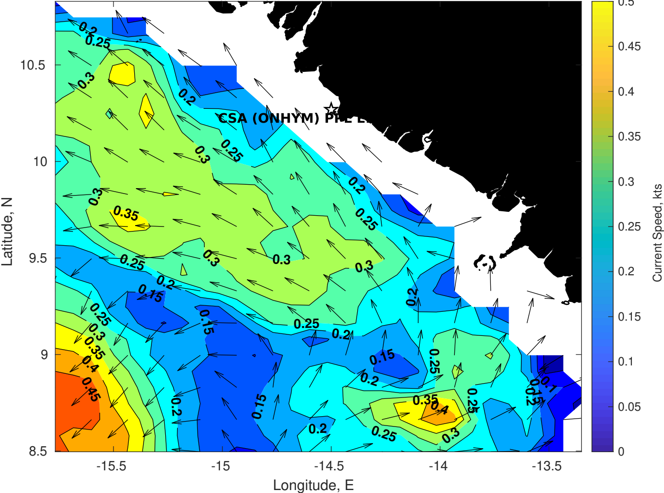
Surface Currents for CSA (ONHYM) PPL EBS - Guinea at 11-Jan-2026 00:00:00
