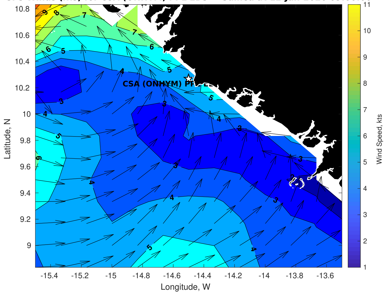
GFS Winds (kts) for CSA (ONHYM) PPL EBS - Guinea at 12-Jan-2026 09:00:00
