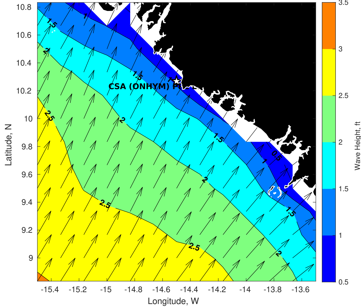
GFS Wave Height (ft) for CSA (ONHYM) PPL EBS - Guinea at 12-Jan-2026 09:00:00
