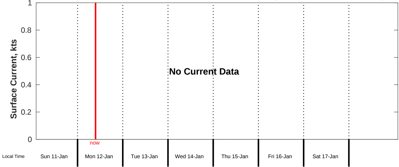
Surface Current Forecast for CSA (ONHYM) PPL EBS - Guinea from 11-Jan-2026 00:00:00 to 19-Jan-2026 00:00:00
