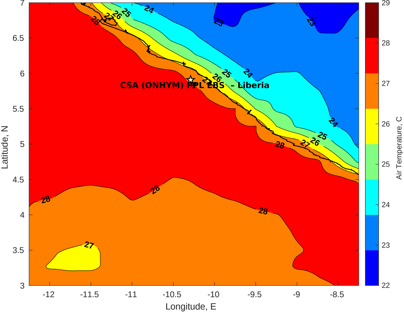
Air Temperature (C) for CSA (ONHYM) PPL EBS - Liberia at 12-Jan-2026
