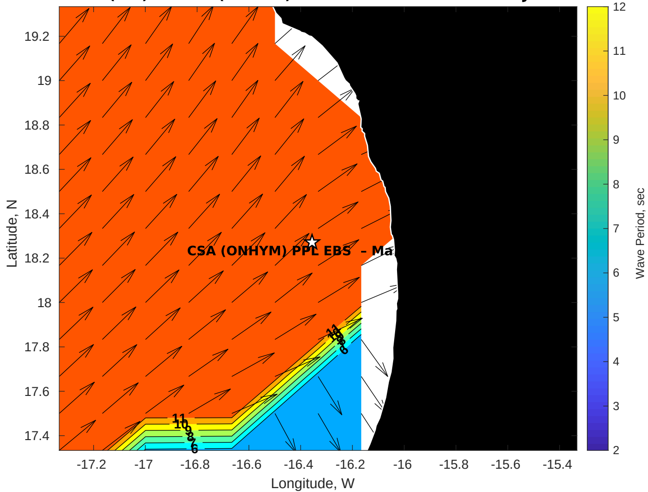
GFS Wave Period (sec) for CSA (ONHYM) PPL EBS - Mauritania at 12-Jan-2026 09:00:00
