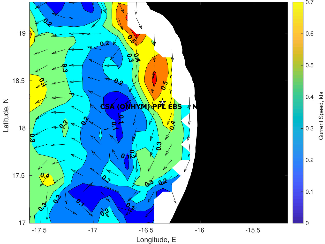
Surface Currents for CSA (ONHYM) PPL EBS - Mauritania at 11-Jan-2026 00:00:00
