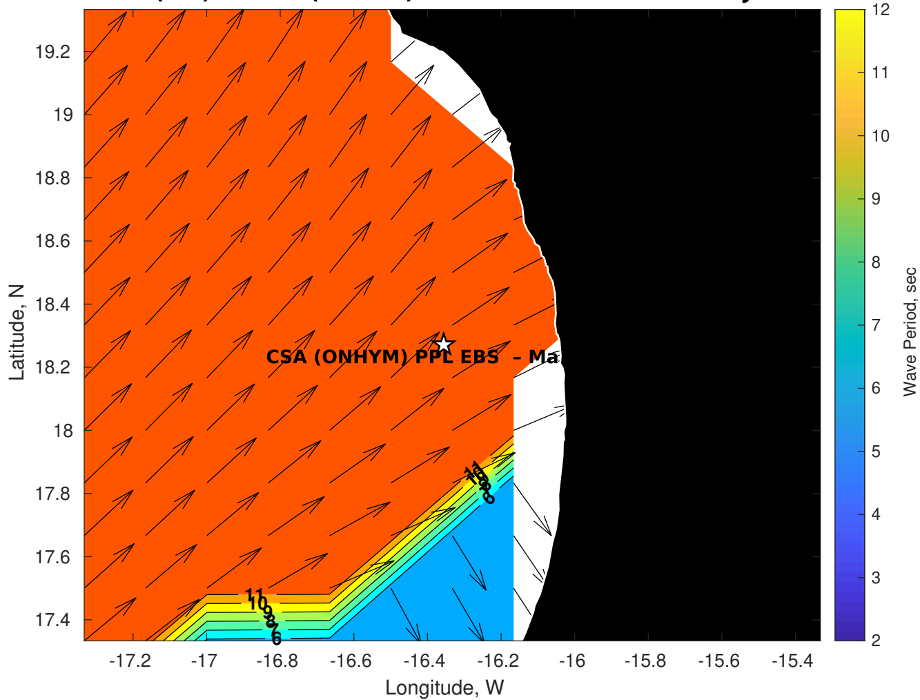
GFS Wave Period (sec) for CSA (ONHYM) PPL EBS - Mauritania at 12-Jan-2026 09:00:00
