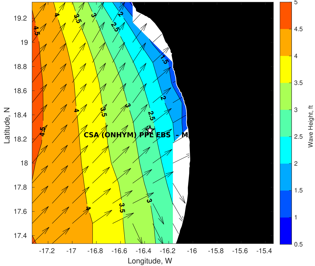
GFS Wave Height (ft) for CSA (ONHYM) PPL EBS - Mauritania at 12-Jan-2026 09:00:00
