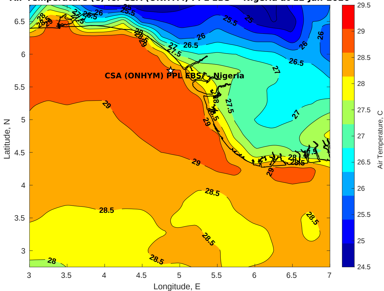
Air Temperature (C) for CSA (ONHYM) PPL EBS - Nigeria at 12-Jan-2026
