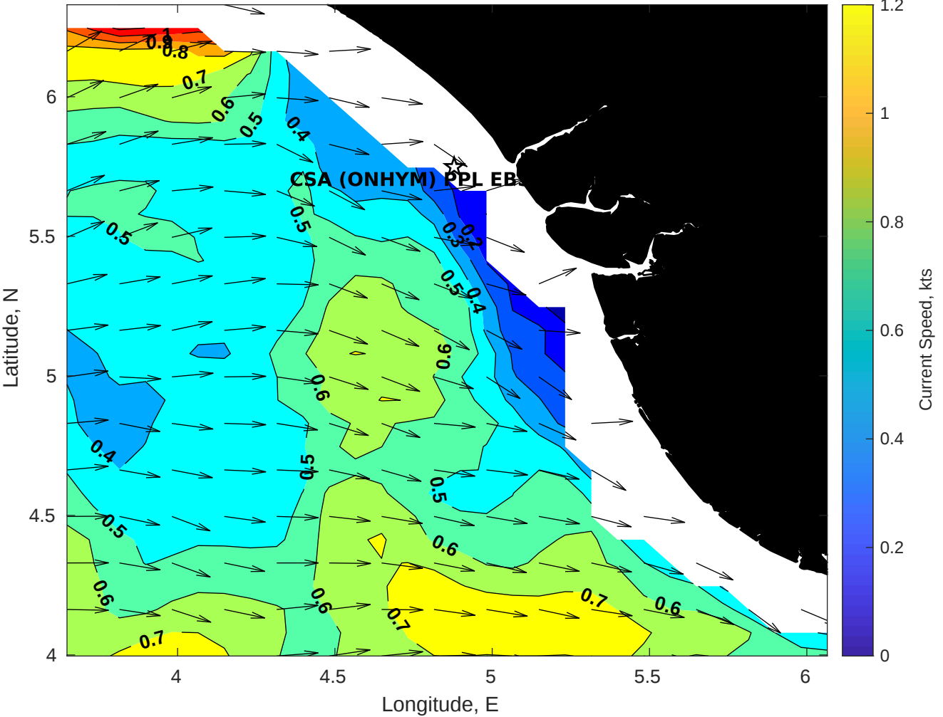
Surface Currents for CSA (ONHYM) PPL EBS - Nigeria at 11-Jan-2026 00:00:00
