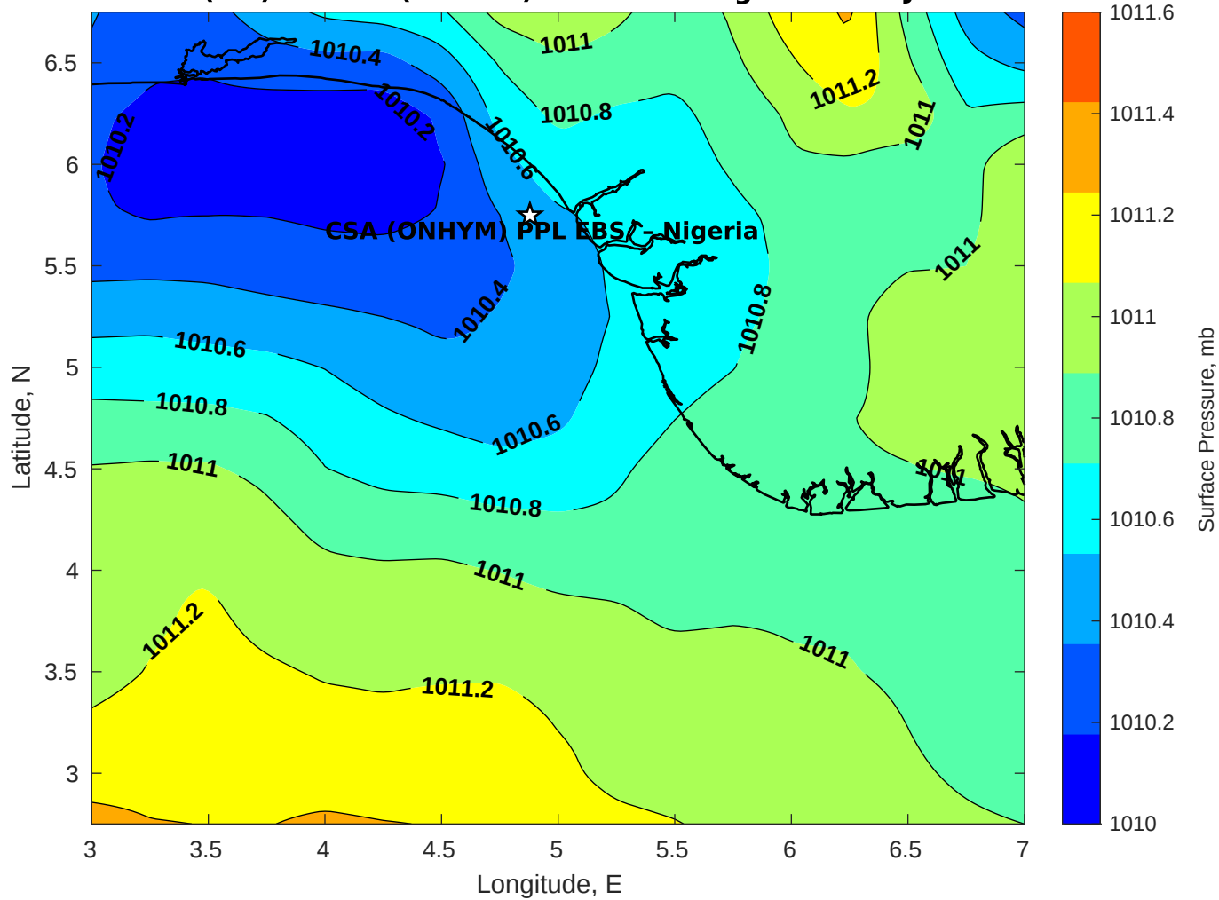
Surface Pressure (mb) for CSA (ONHYM) PPL EBS - Nigeria at 12-Jan-2026 00:00:00
