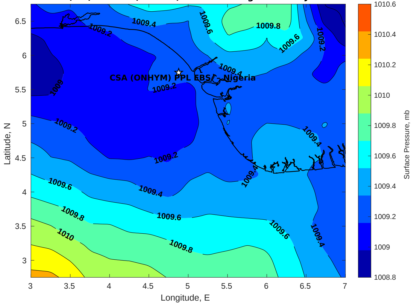
Surface Pressure (mb) for CSA (ONHYM) PPL EBS - Nigeria at 14-Jan-2026 00:00:00
