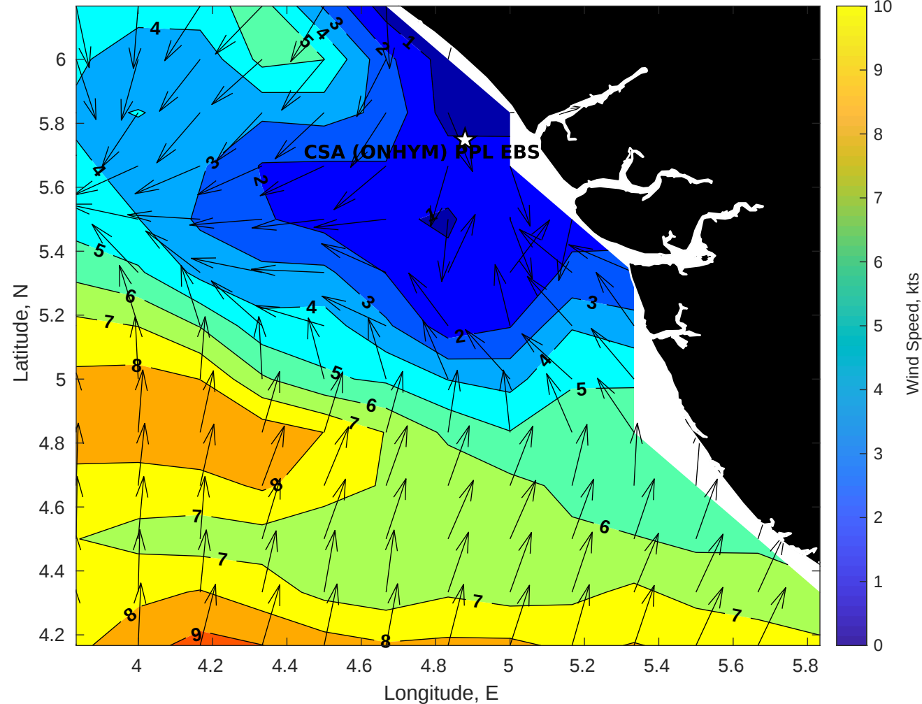
GFS Winds (kts) for CSA (ONHYM) PPL EBS - Nigeria at 12-Jan-2026 09:00:00
