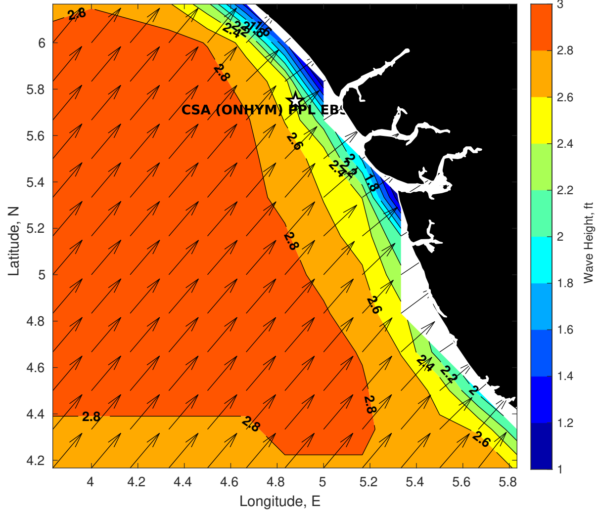
GFS Wave Height (ft) for CSA (ONHYM) PPL EBS - Nigeria at 12-Jan-2026 09:00:00
