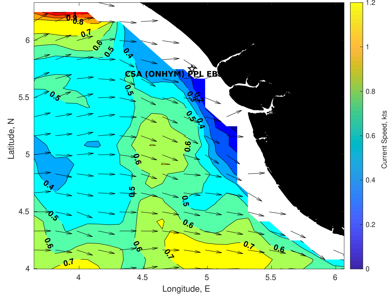
Surface Currents for CSA (ONHYM) PPL EBS - Nigeria at 11-Jan-2026 00:00:00
