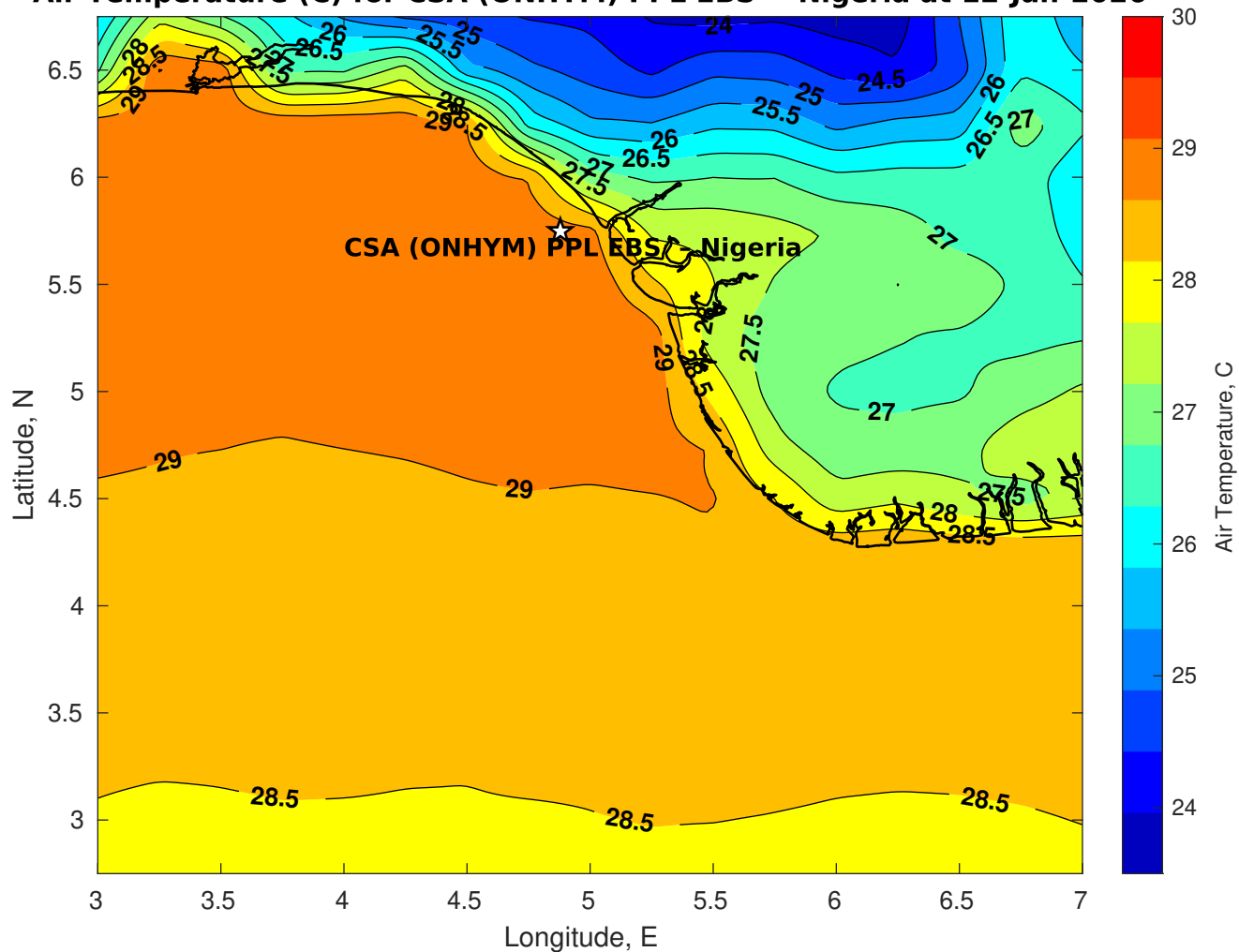
Air Temperature (C) for CSA (ONHYM) PPL EBS - Nigeria at 12-Jan-2026
