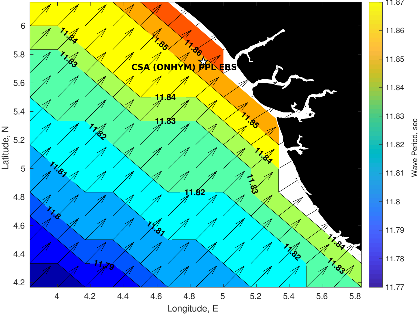
GFS Wave Period (sec) for CSA (ONHYM) PPL EBS - Nigeria at 12-Jan-2026 09:00:00
