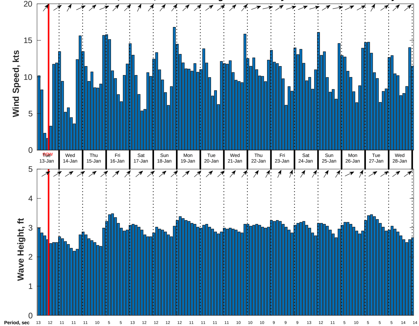
Wind & Wave Forecast for CSA (ONHYM) PPL EBS - Nigeria from 12-Jan-2026 02:00:00 to 28-Jan-2026 02:00:00
