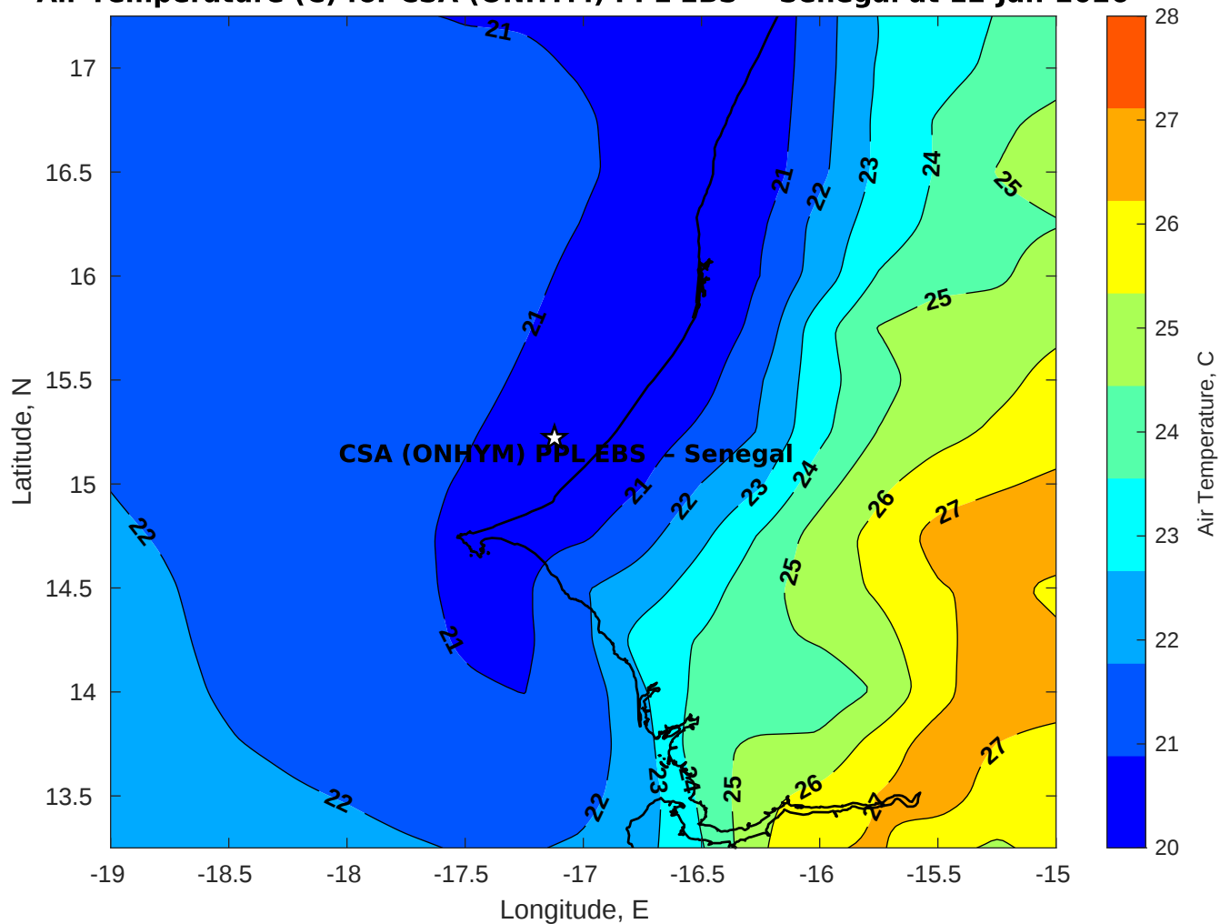
Air Temperature (C) for CSA (ONHYM) PPL EBS - Senegal at 12-Jan-2026
