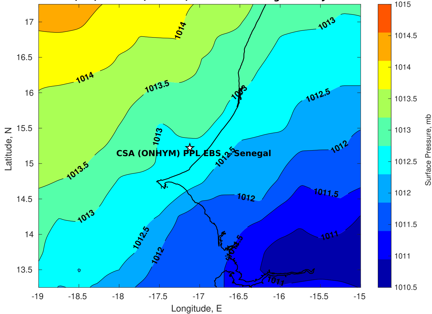
Surface Pressure (mb) for CSA (ONHYM) PPL EBS - Senegal at 13-Jan-2026 00:00:00
