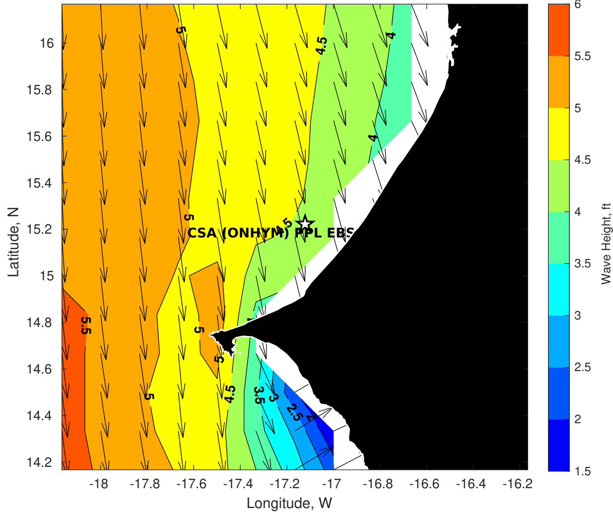
GFS Wave Height (ft) for CSA (ONHYM) PPL EBS - Senegal at 12-Jan-2026 09:00:00
