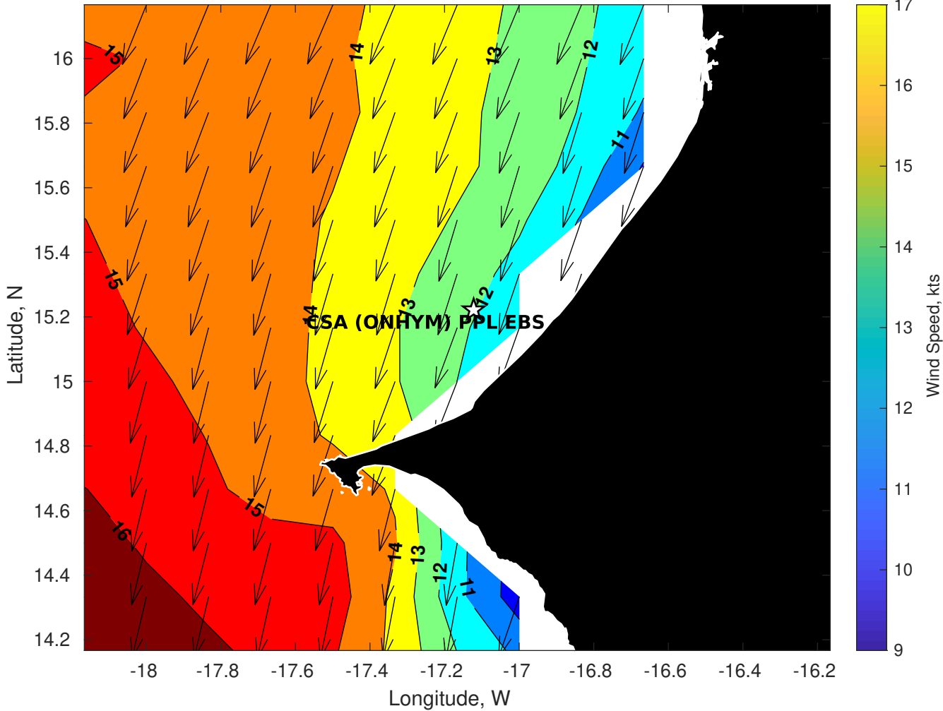
GFS Winds (kts) for CSA (ONHYM) PPL EBS - Senegal at 12-Jan-2026 09:00:00
