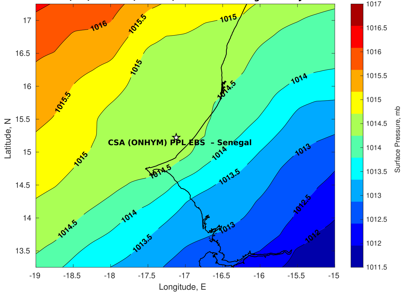
Surface Pressure (mb) for CSA (ONHYM) PPL EBS - Senegal at 12-Jan-2026 00:00:00
