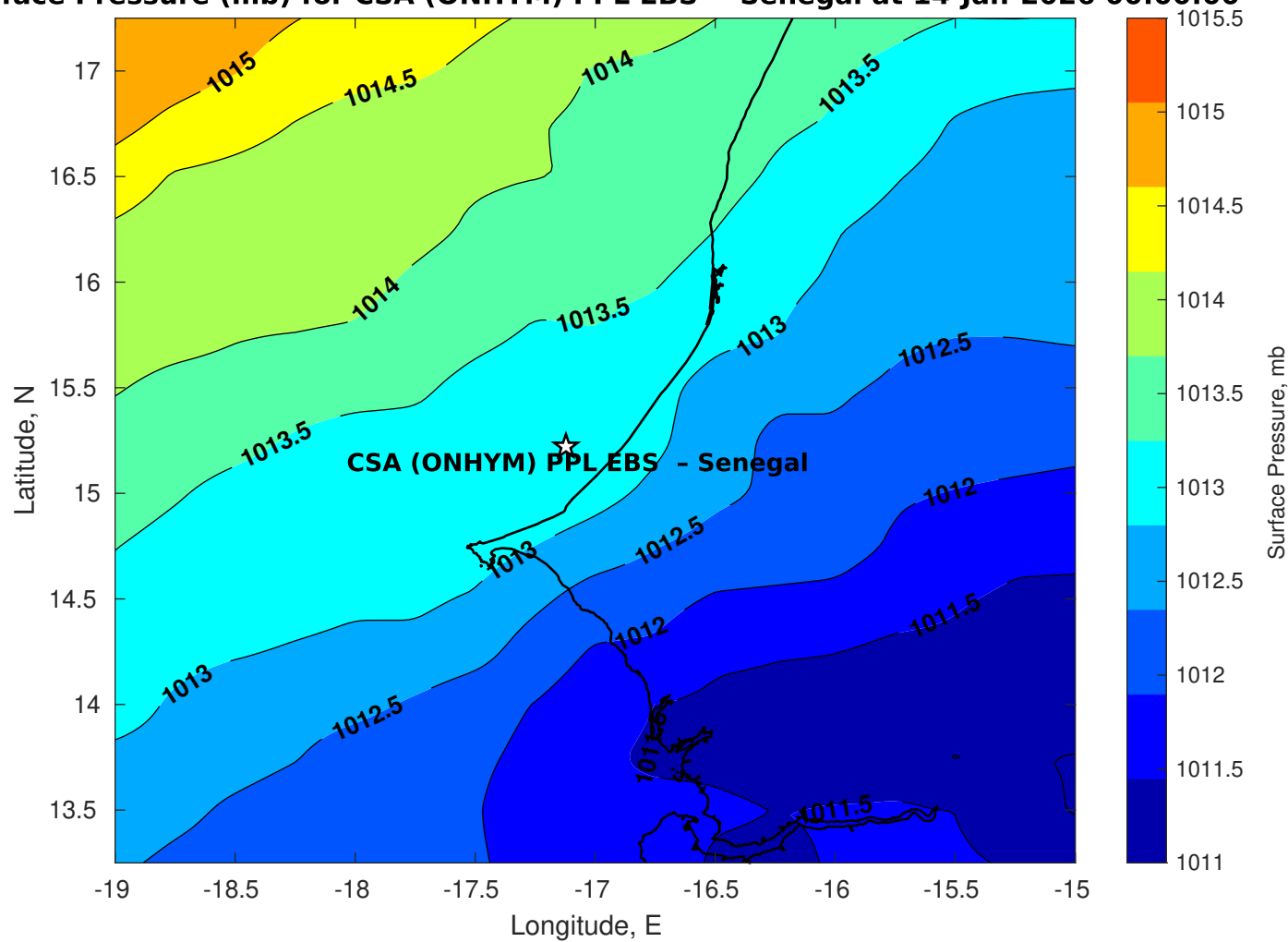
Surface Pressure (mb) for CSA (ONHYM) PPL EBS - Senegal at 14-Jan-2026 00:00:00
