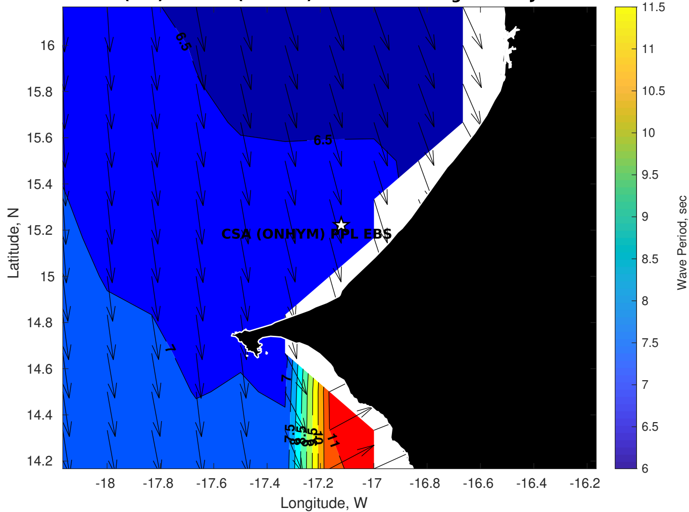
GFS Wave Period (sec) for CSA (ONHYM) PPL EBS - Senegal at 12-Jan-2026 09:00:00
