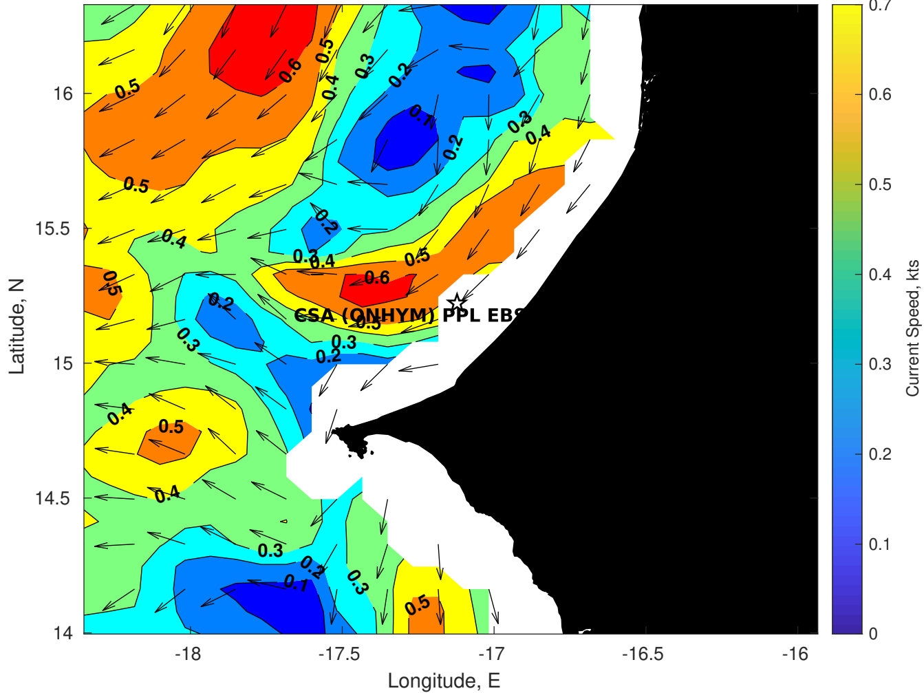
Surface Currents for CSA (ONHYM) PPL EBS - Senegal at 11-Jan-2026 00:00:00
