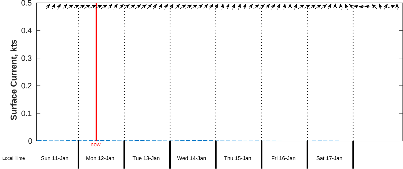
Surface Current Forecast for CSA (ONHYM) PPL EBS - Senegal from 11-Jan-2026 00:00:00 to 19-Jan-2026 00:00:00
