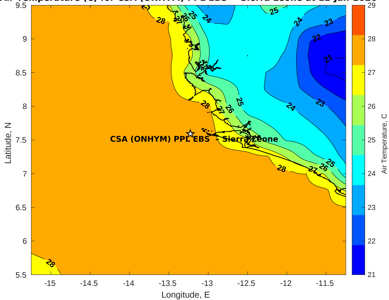
Air Temperature (C) for CSA (ONHYM) PPL EBS - Sierra Leone at 12-Jan-2026
