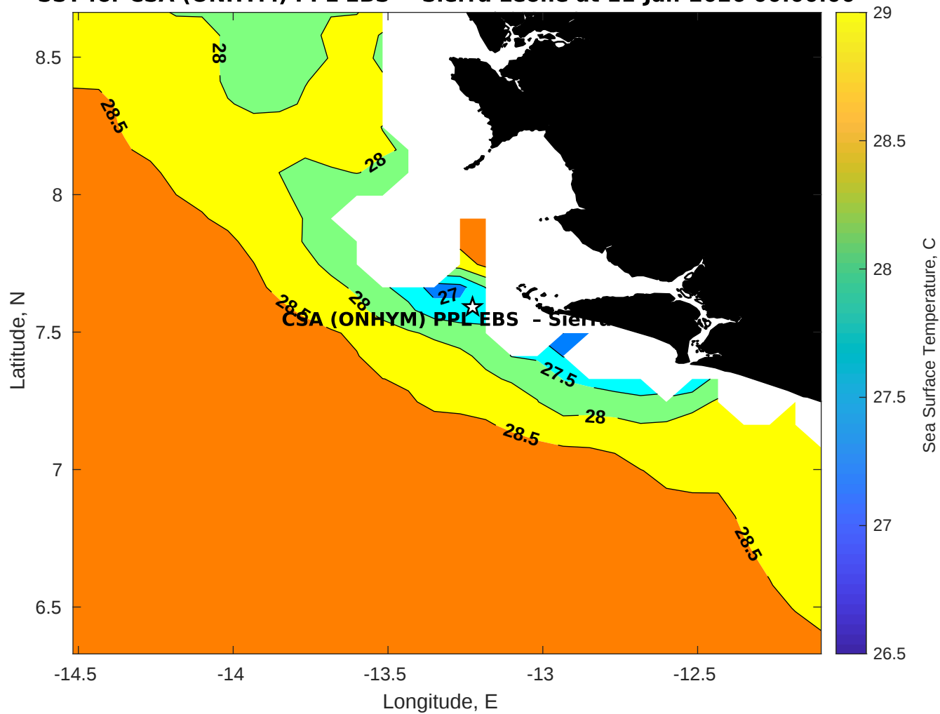
SST for CSA (ONHYM) PPL EBS - Sierra Leone at 11-Jan-2026 00:00:00
