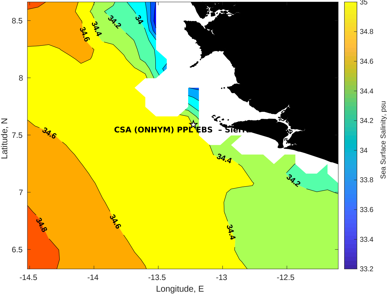
Surface Salinity for CSA (ONHYM) PPL EBS - Sierra Leone at 11-Jan-2026 00:00:00
