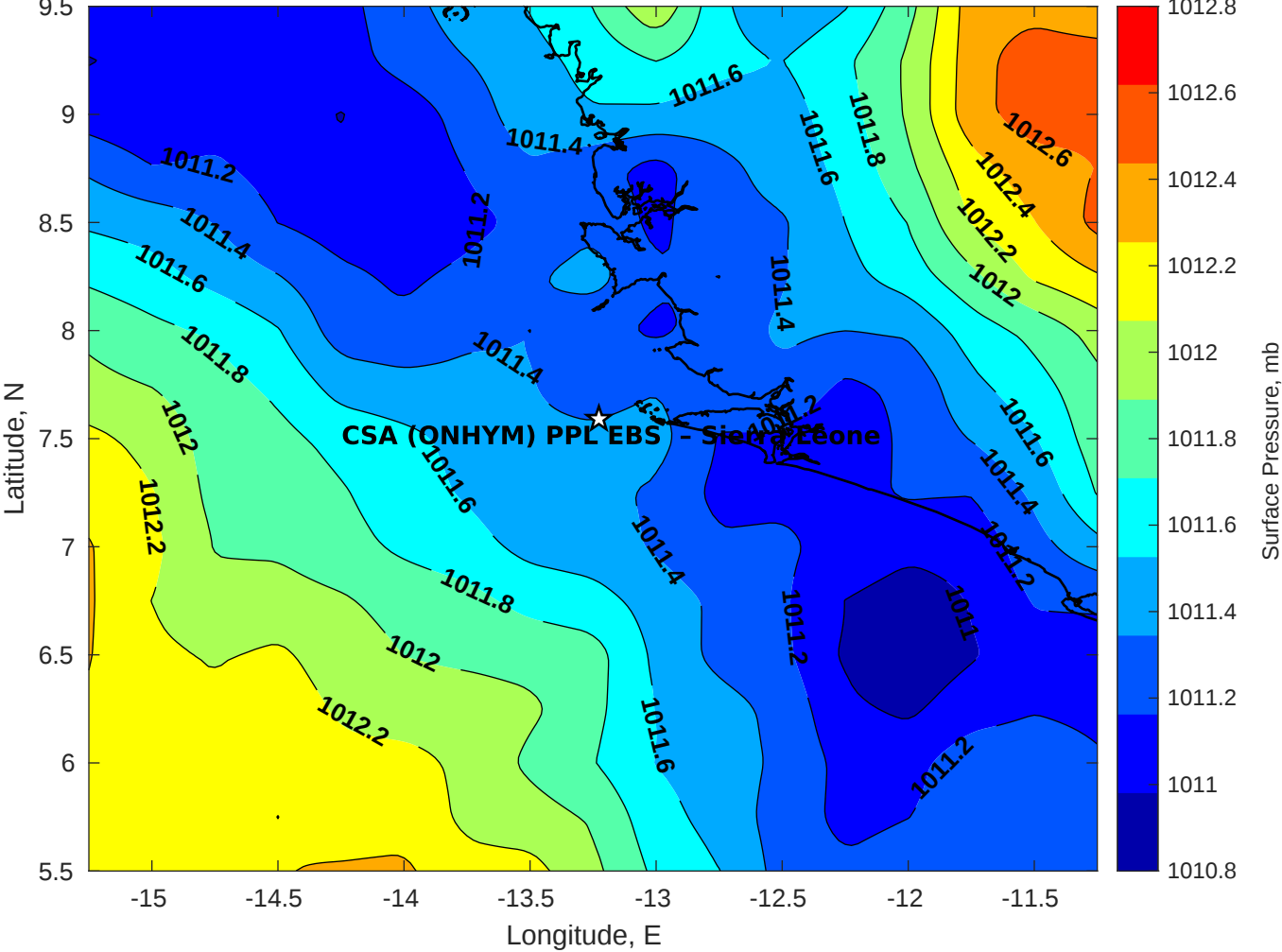
Surface Pressure (mb) for CSA (ONHYM) PPL EBS - Sierra Leone at 13-Jan-2026 00:00:00
