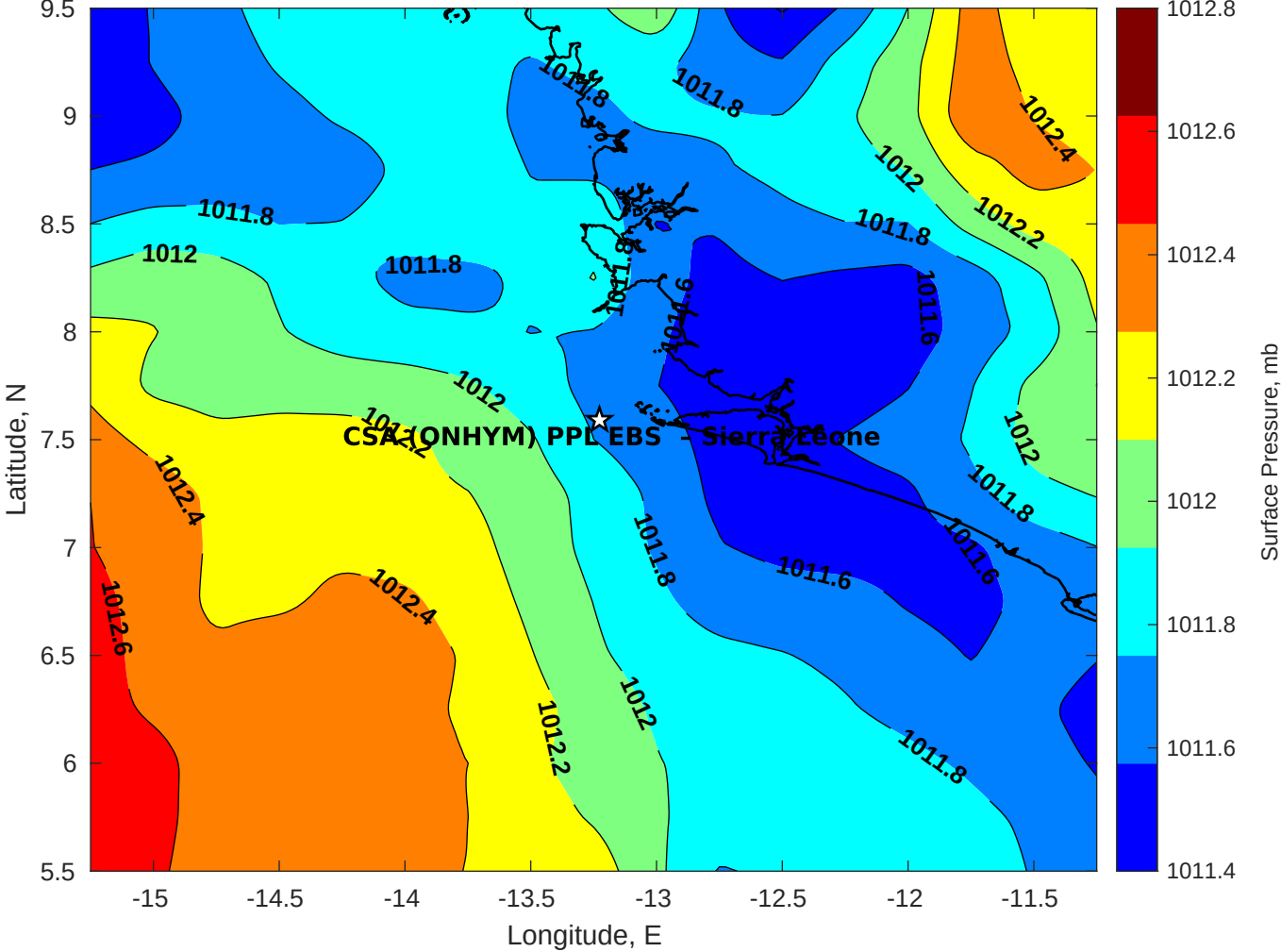
Surface Pressure (mb) for CSA (ONHYM) PPL EBS - Sierra Leone at 14-Jan-2026 00:00:00
