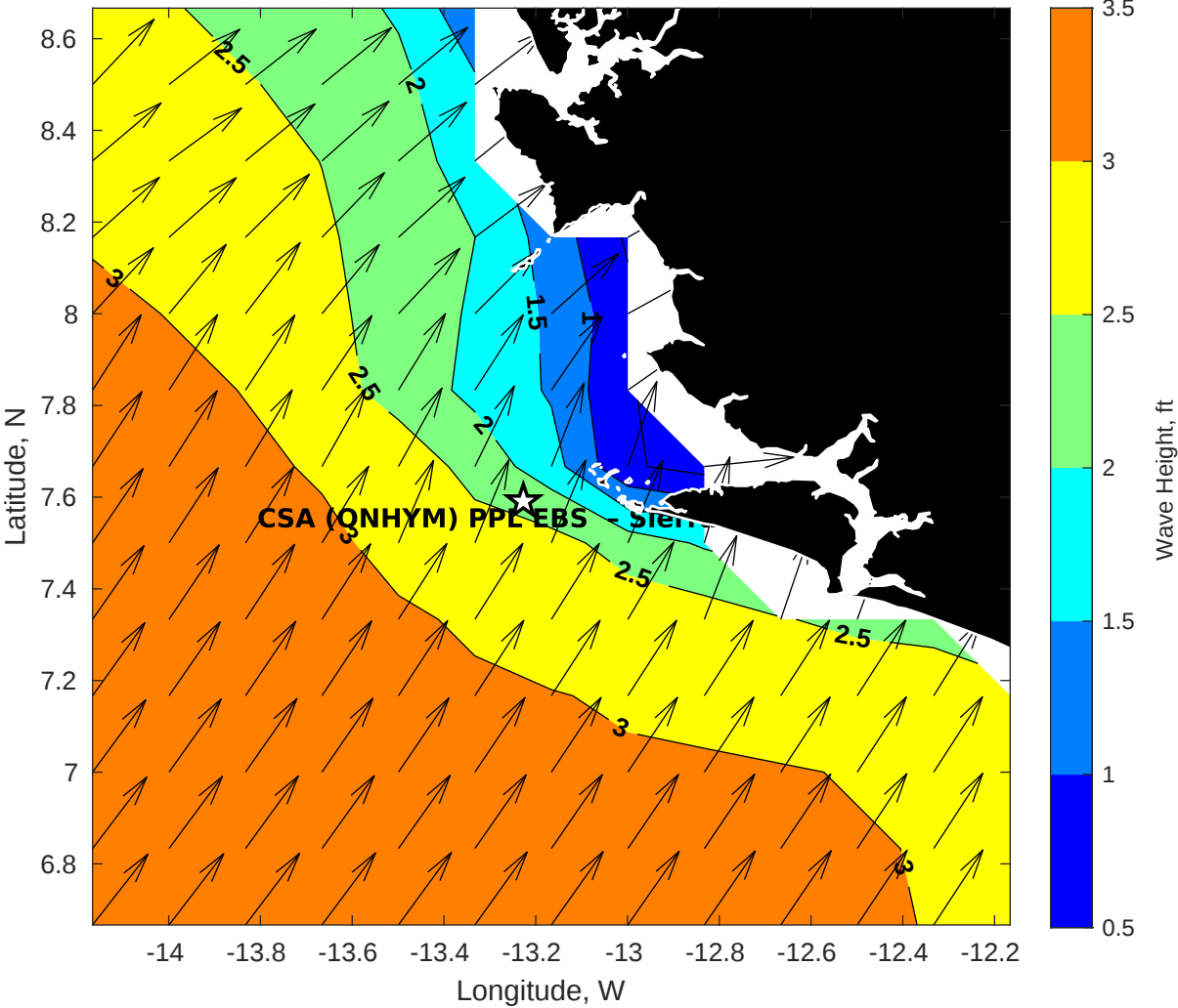
GFS Wave Height (ft) for CSA (ONHYM) PPL EBS - Sierra Leone at 12-Jan-2026 09:00:00
