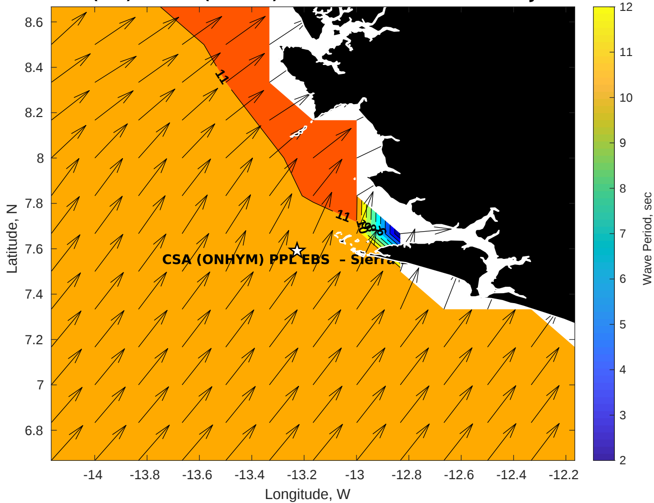
GFS Wave Period (sec) for CSA (ONHYM) PPL EBS - Sierra Leone at 12-Jan-2026 09:00:00
