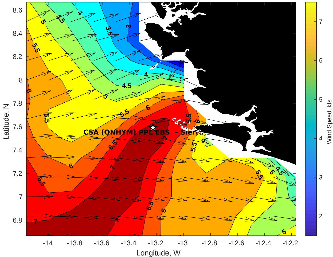
GFS Winds (kts) for CSA (ONHYM) PPL EBS - Sierra Leone at 12-Jan-2026 09:00:00
