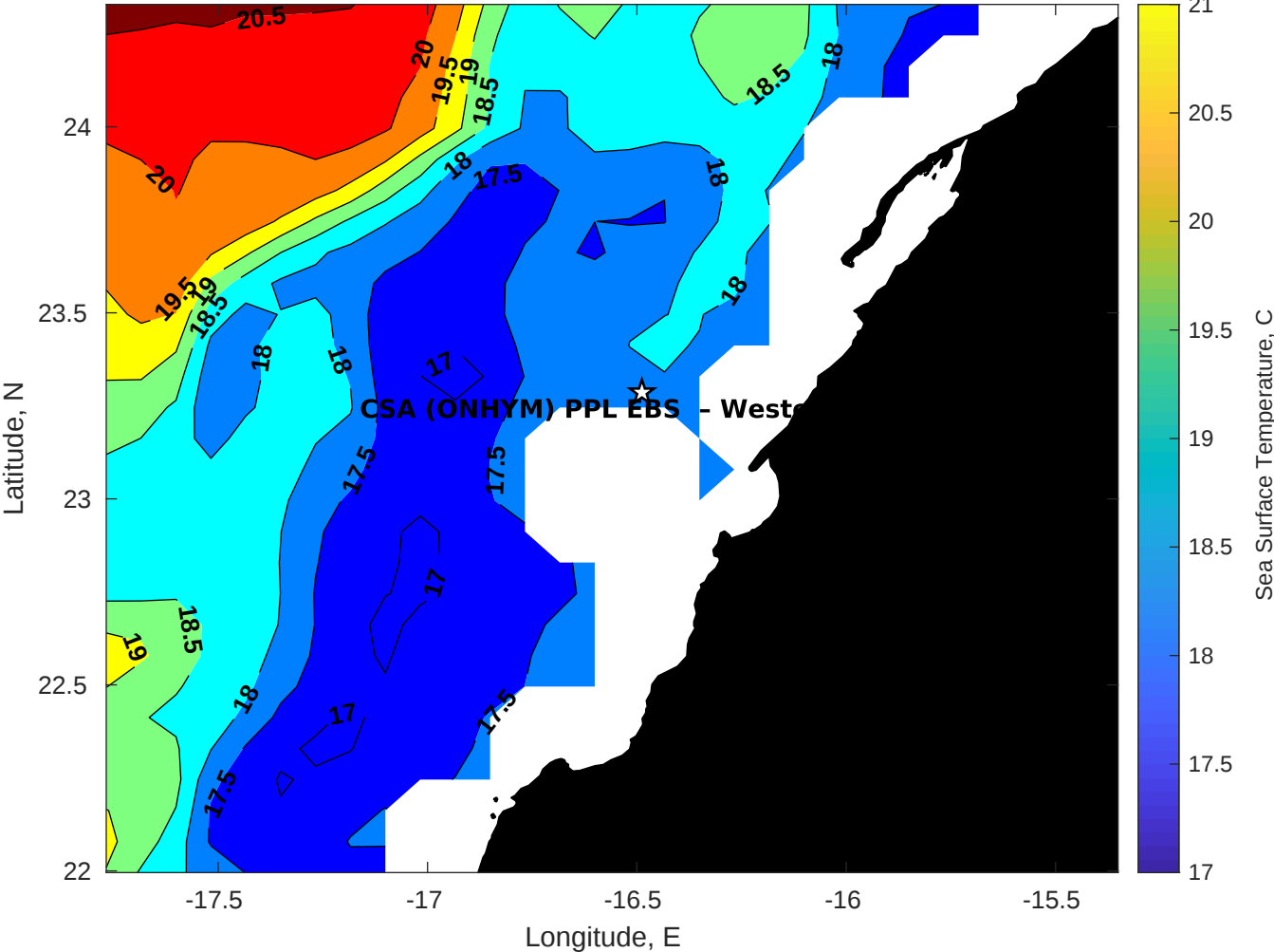
SST for CSA (ONHYM) PPL EBS - Western Sahara at 11-Jan-2026 00:00:00
