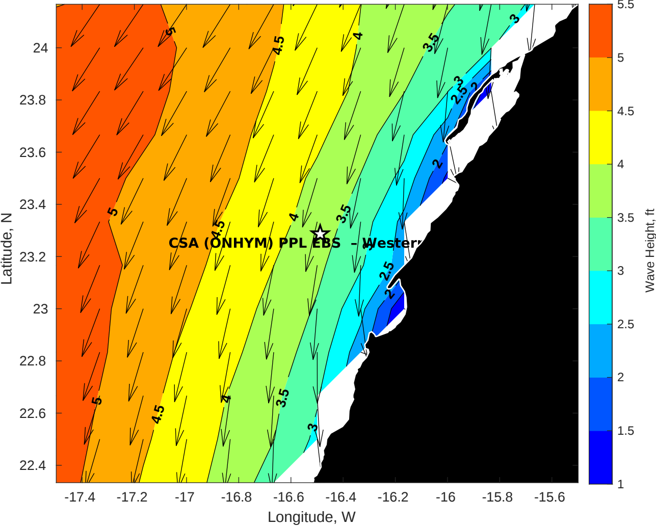
GFS Wave Height (ft) for CSA (ONHYM) PPL EBS - Western Sahara at 12-Jan-2026 09:00:00
