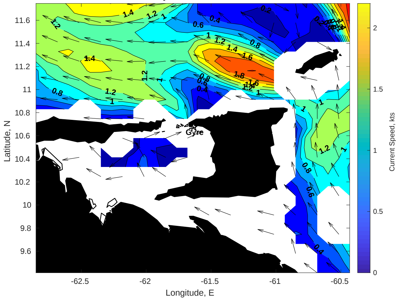
Surface Currents for Gyre at 11-Jan-2026 00:00:00
