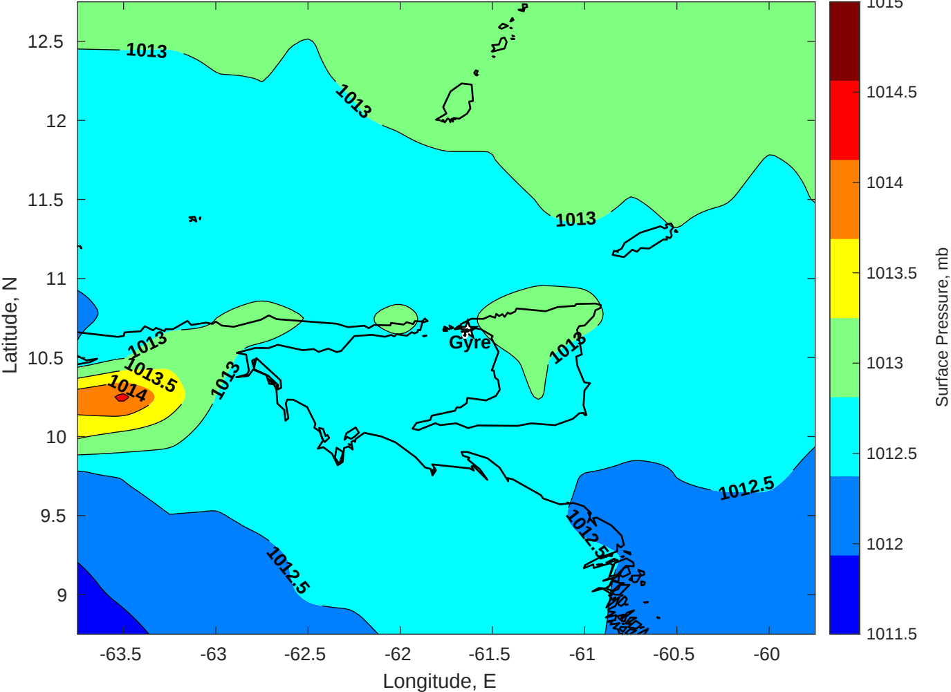
Surface Pressure (mb) for Gyre at 12-Jan-2026 00:00:00
