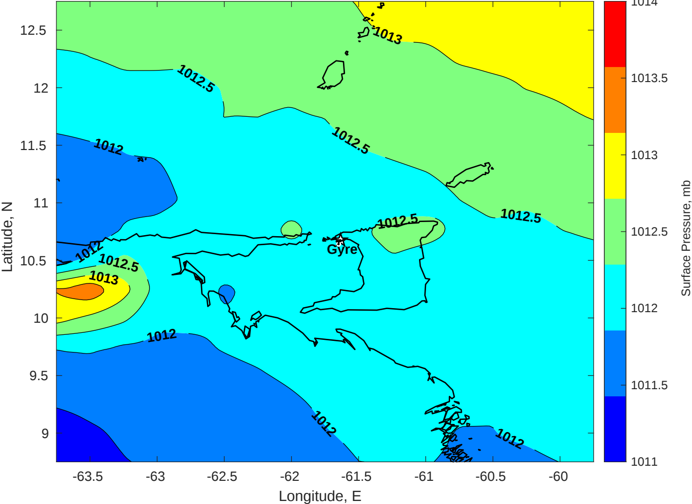
Surface Pressure (mb) for Gyre at 14-Jan-2026 00:00:00
