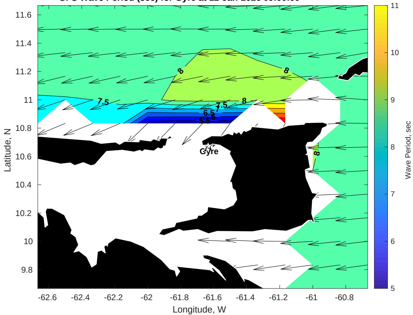
GFS Wave Period (sec) for Gyre at 12-Jan-2026 09:00:00
