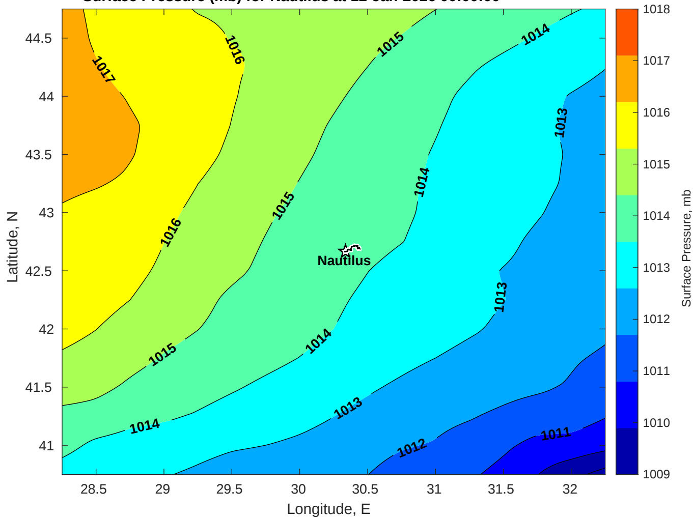
Surface Pressure (mb) for Nautilus at 12-Jan-2026 00:00:00
